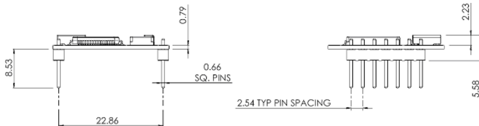
Figure 3. Side Views
